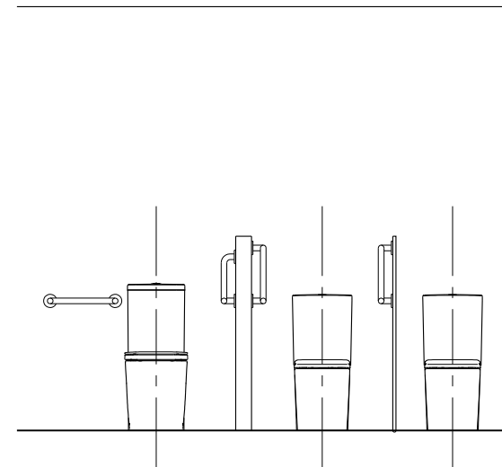
SECTION C.C.
