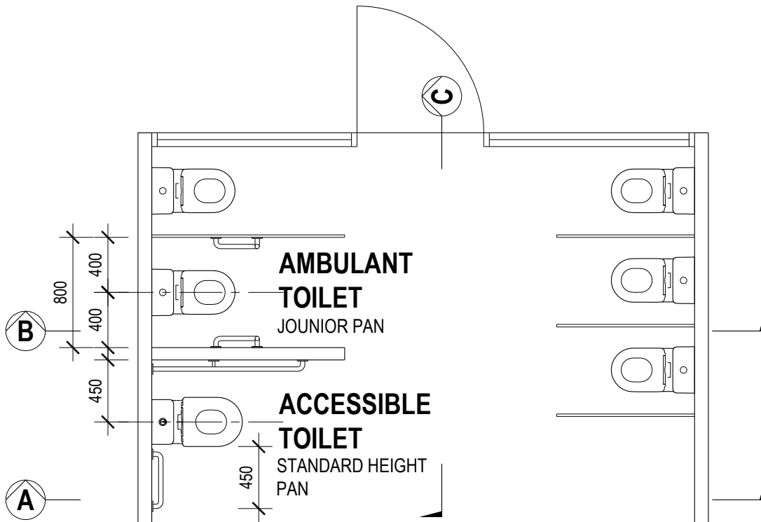
PROPOSED PLAN
